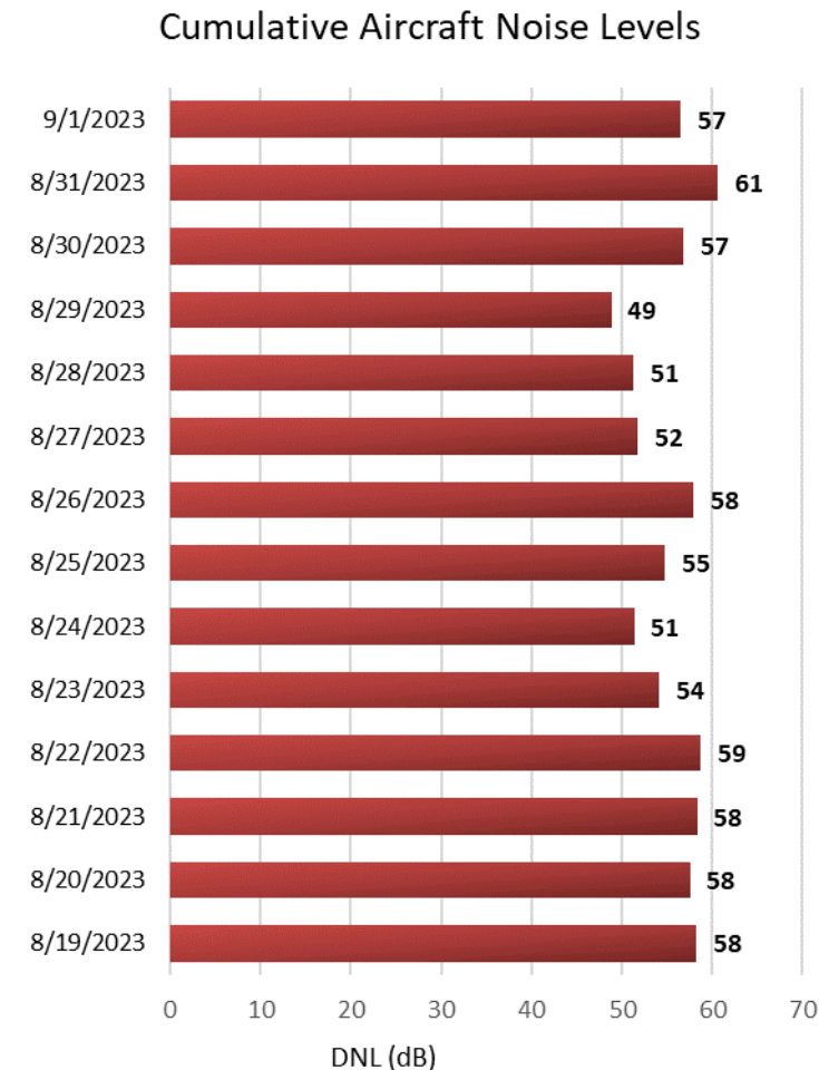
Figure 10. Measured Daily Aircraft Noise Levels
