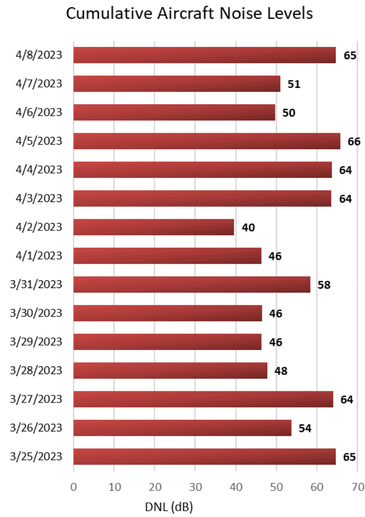
Figure 10. Measured Daily Aircraft Noise Levels
