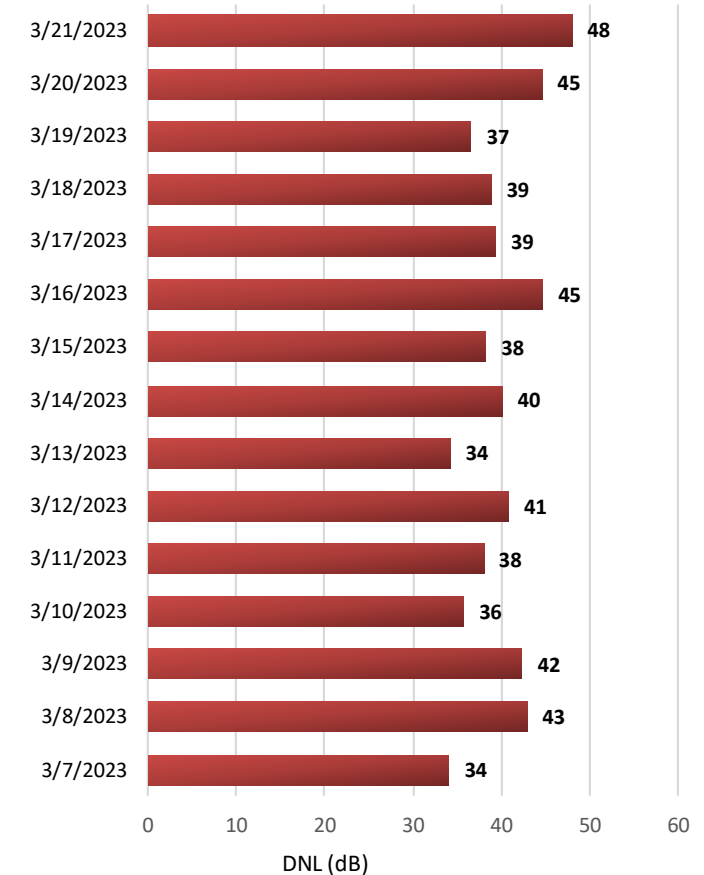
Cumulative Aircraft Noise Levels
