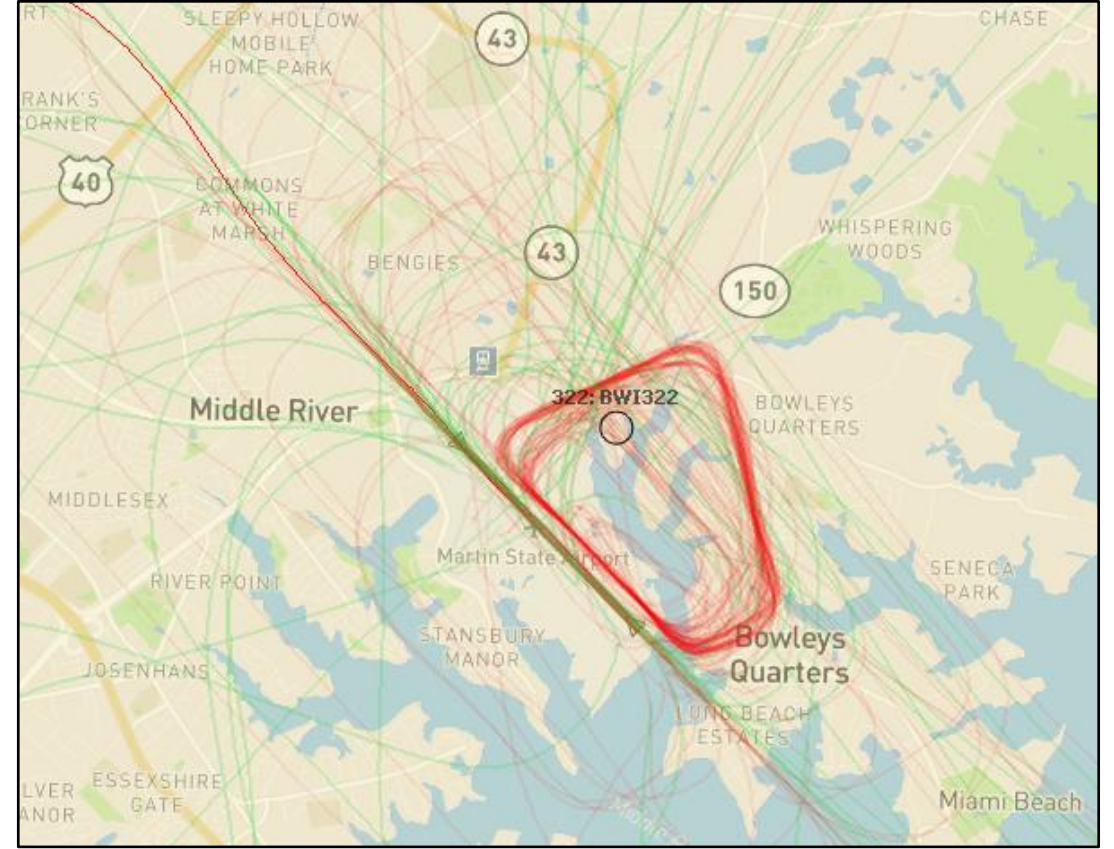
Figure 5. All Martin State Airport Arrivals and Departures Correlated to Aircraft Noise Events During the Measurement Period (Green = Departures, Red = Arrivals)
