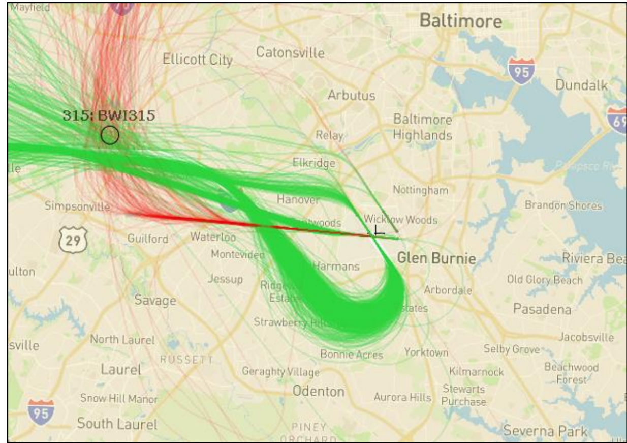
Figure 5. All BWI Marshall Arrivals and Departures Correlated to Aircraft Noise Events During the Measurement Period (Green = Departures, Red = Arrivals)
