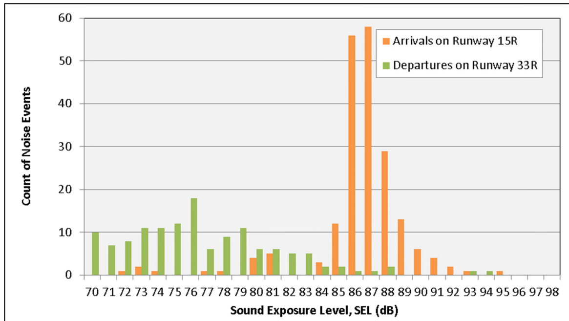
Figure 10. Counts of Sound Exposure Levels from Aircraft Overflights over the Full Measurement Period – Departures on Runways 33R and Arrivals on Runway 15R
