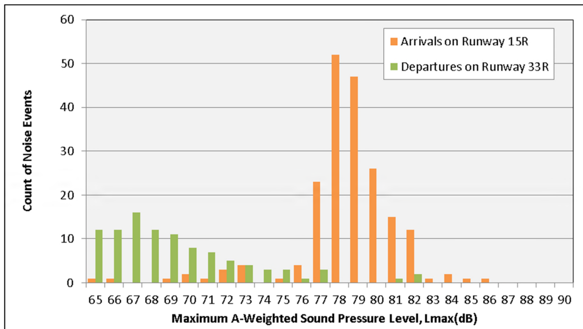
Figure 8. Counts of Maximum Noise Levels from Aircraft Overflights over the Full Measurement Period – Departures on Runway 33R and Arrivals on Runway 15R
